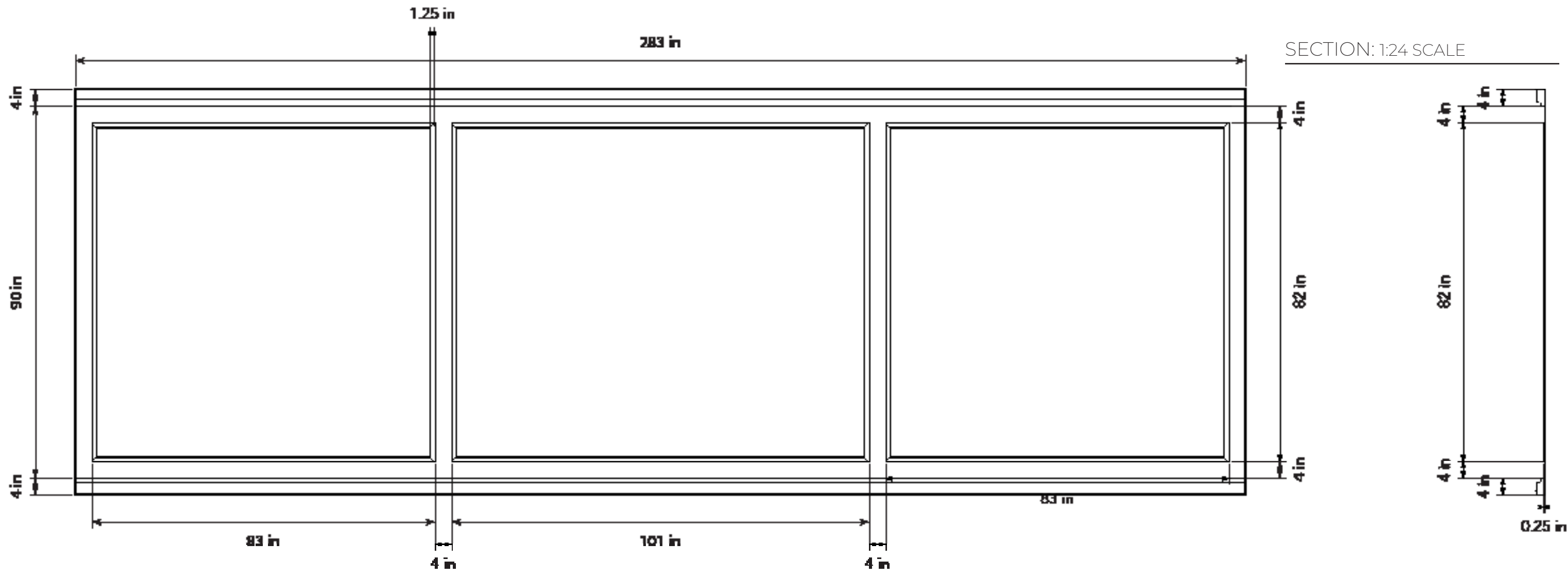
ELEVATION: 1:24 SCALE
